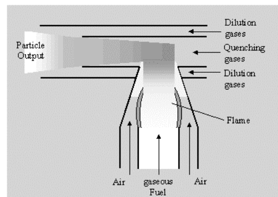
Fig. 1: Schematic of Jing-CAST burner [1]
