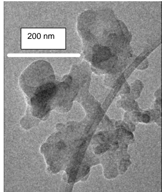
Fig. 7: TEM picture of "solid like" large soot particles from CAST burner
